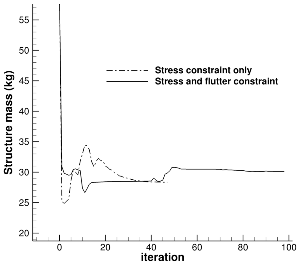
Figure 5.1: Algorithm converge curve with and without flutter constraint
